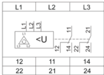
Wiring Diagram
